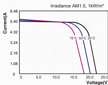
I-V Curves of PV module SOL-SYS90W at various cell temperatures
