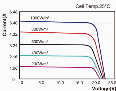
I-V Curves of PV module SOL-SYS90W
